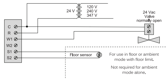
Connection layout for a hot water valve
