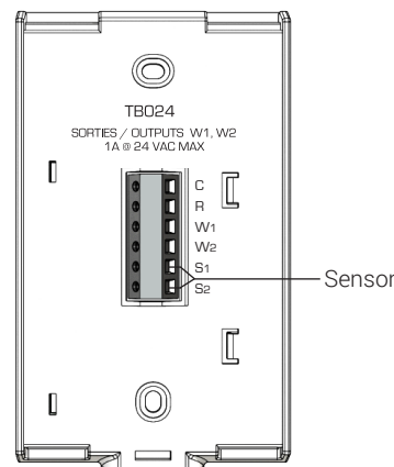
Connection of the floor sensor (optional)
