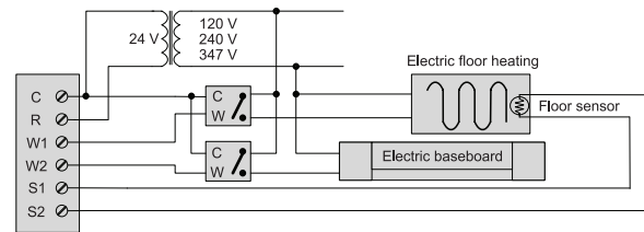
Connection layout for an electric floor heating with electric baseboard on the 2nd heating stage
