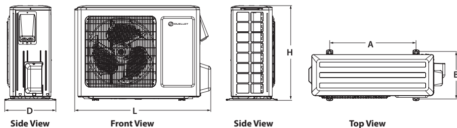
Side View
