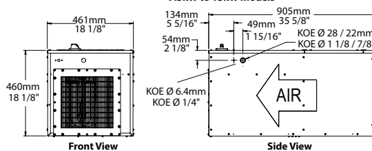
Dimensions for ductwork
