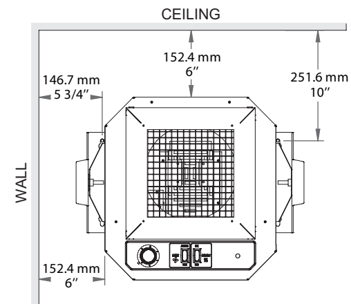
Figure 2 Minimum clearance:
