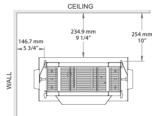
Figure 3 Minimum Clearance:
