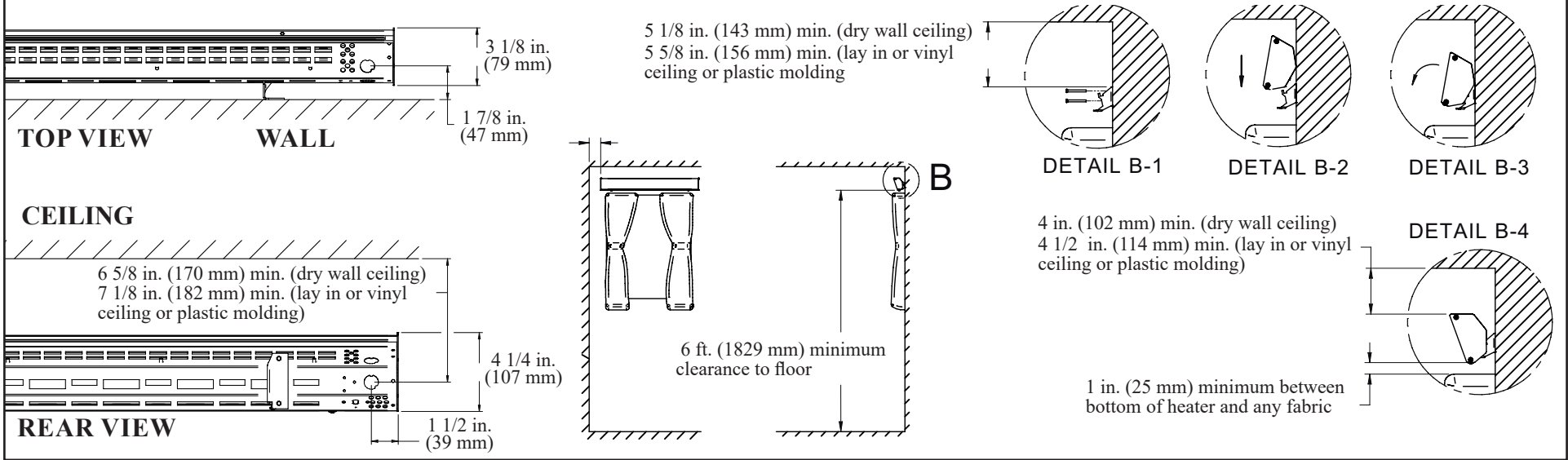
Figure 4 - MOUNTING RESTRICTIONS
