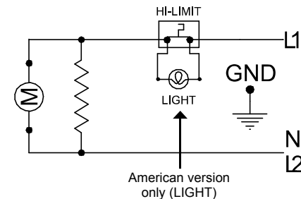
120V, 208V, 240V Wiring Diagram
