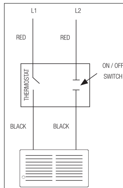
Double-pole Installation
